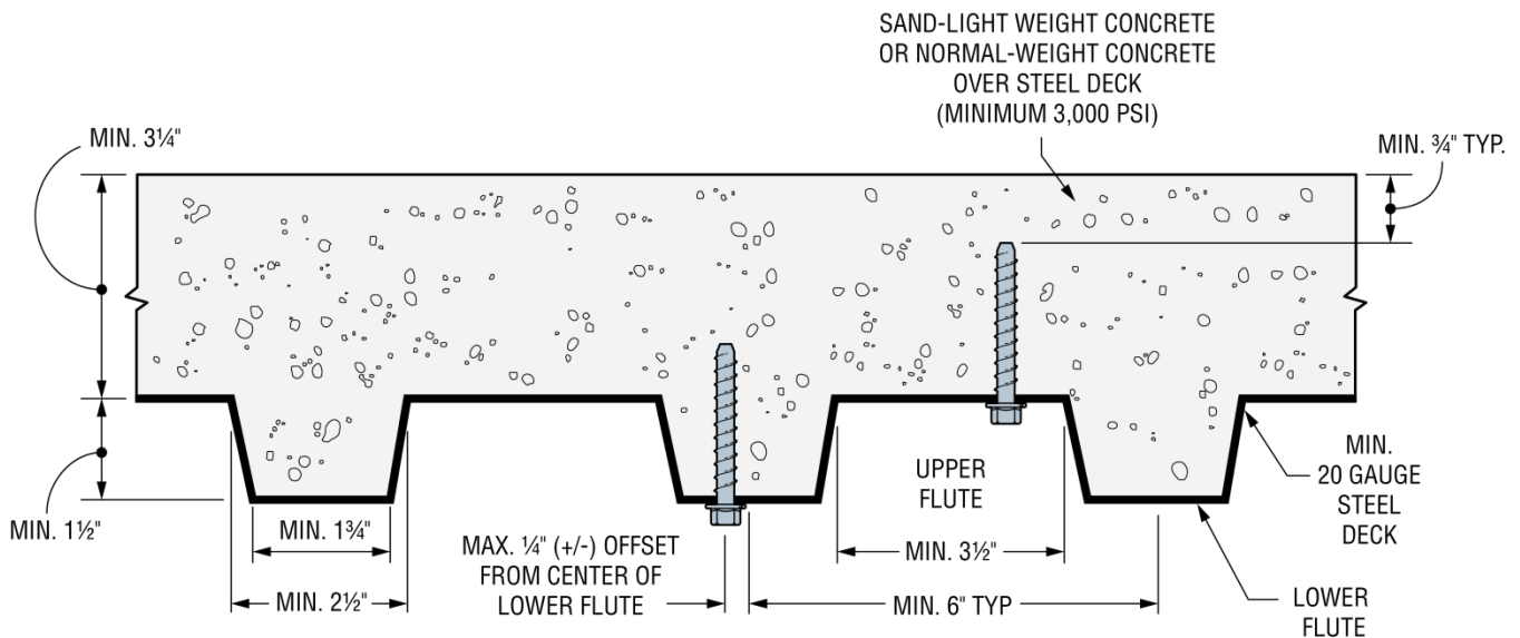
FIGURE 4—INSTALLATION OF \frac{1}{4} -INCH SHANK DIAMETER SCREW ANCHORS AND ROD HANGERS INTO THE SOFFIT OF CONCRETE-FILLED PROFILE STEEL DECK FLOOR AND ROOF ASSEMBLIES (1 in = 25.4 mm)
