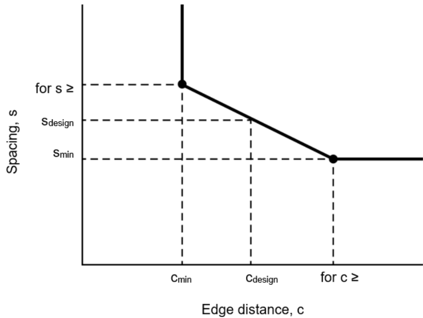
FIGURE 2D— INTERPOLATION OF MINIMUM EDGE DISTANCE AND ANCHOR SPACING 1
